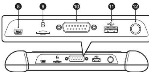
Figure 2-3 MaxiIM Tablet, Top View
